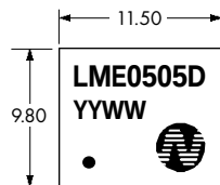
8 Pin DIP
