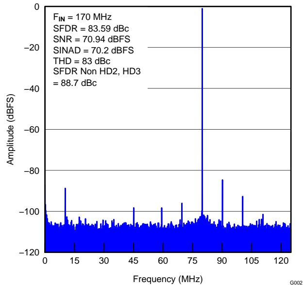
Figure 14. INPUT SIGNAL (170 MHz)
