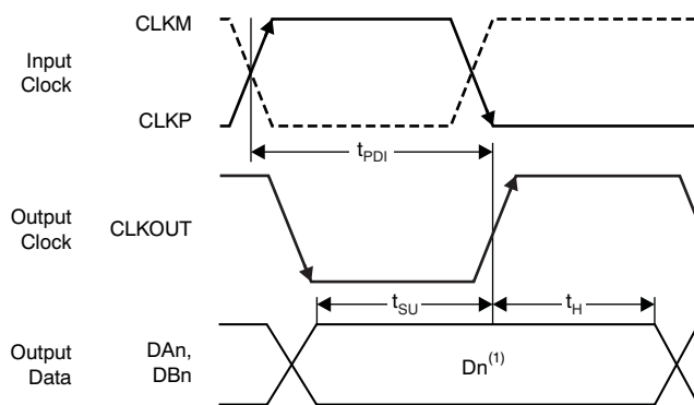
Figure 3. CMOS Interface Timing Diagram
