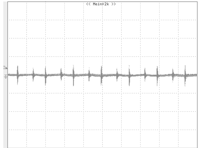
Figure 12: Input reflected ripple current, i_s , through a 12\mu\text{H} source inductor at nominal input voltage and rated load current (50 mA/div, 2 \mu\text{s} /div)
