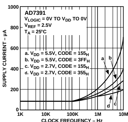
Figure 12. Supply Current vs. Clock Frequency
