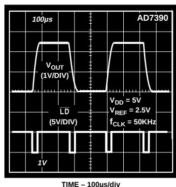
Figure 17. Large Signal Settling Time
