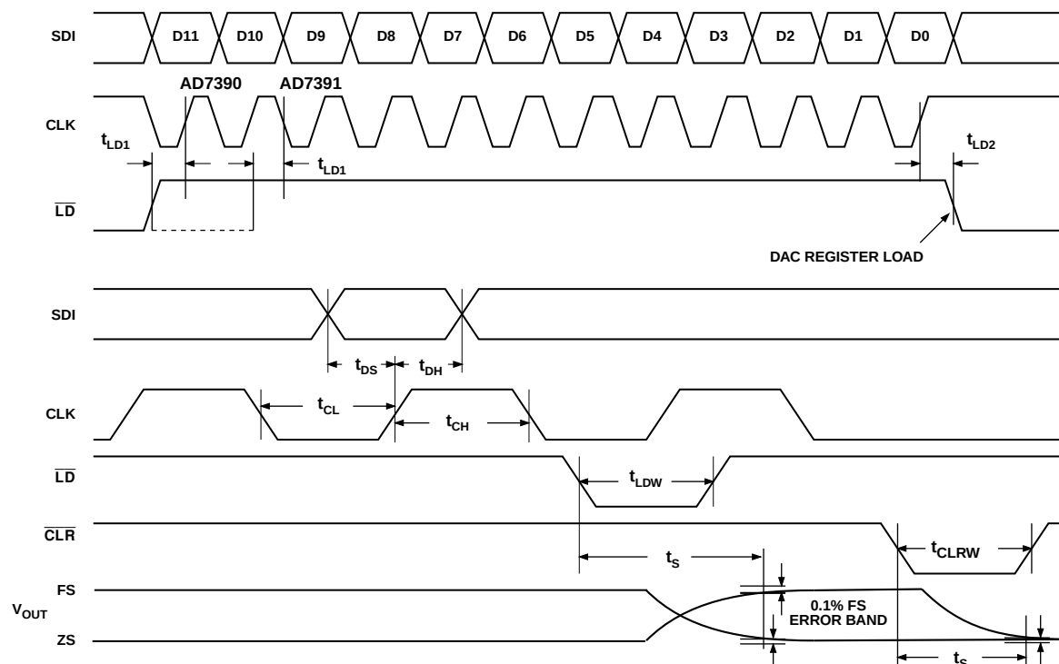
Figure 4. Timing Diagram
