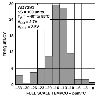
Figure 7. AD7391 Full-Scale Output Tempco Histogram
