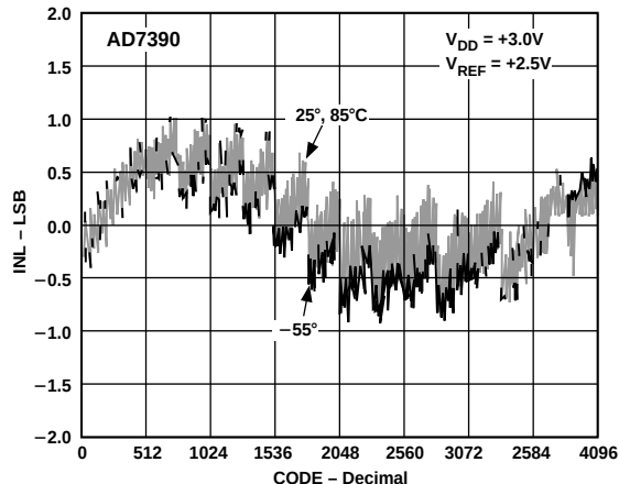
Figure 2. INL Error vs. Code & Temperature
