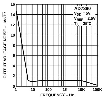
Figure 8. Voltage Noise Density vs. Frequency
