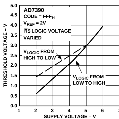
Figure 10. Logic Threshold vs. Supply Voltage
