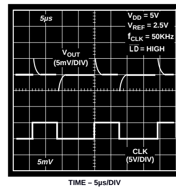
Figure 16. Digital Feedthrough Performance
