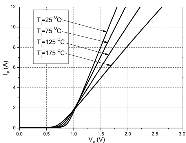
Figure 1. Forward Characteristics
