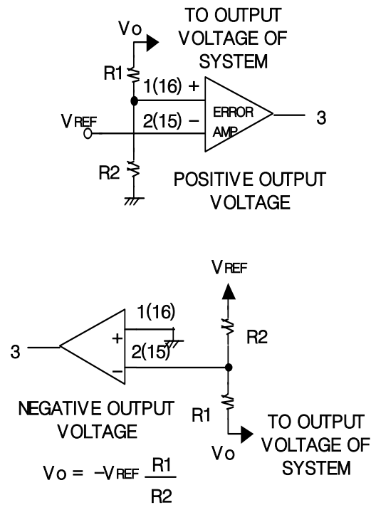
Fig. 7 Error Amplifier Sensing Techniques
