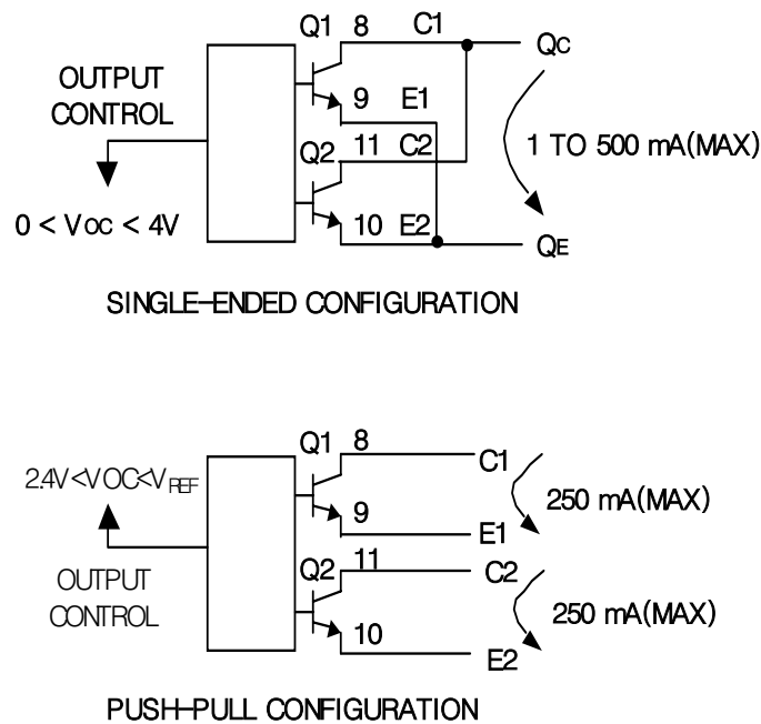
Fig. 6 Output Connections for Single-Ended and Push-Pull Configurations
