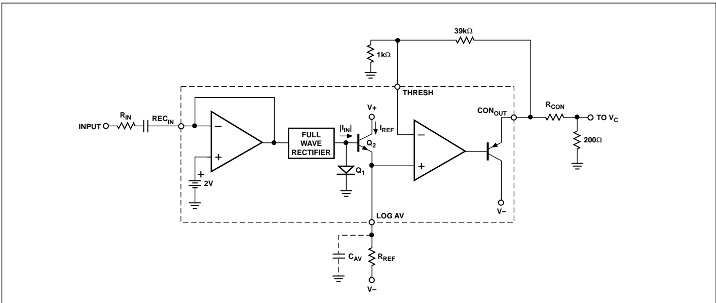
FIGURE 2: Level Detector
