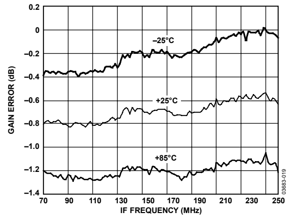
Figure 18. Gain Error vs. Frequency
