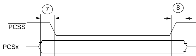
Figure 50. DSPI PCS strobe ( \overline{\text{PCSS}} ) timing
