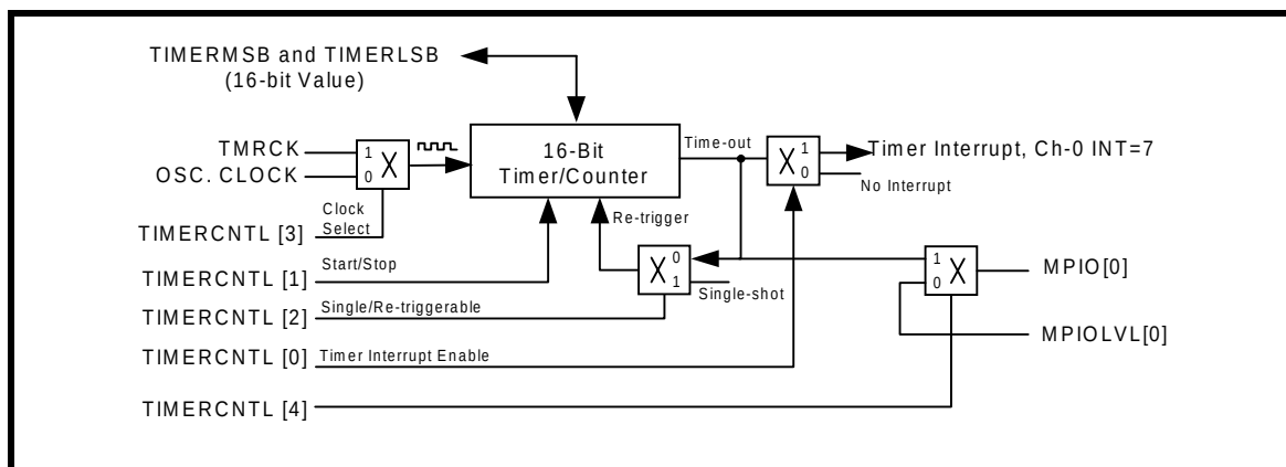
FIGURE 5. TIMER/COUNTER CIRCUIT.
