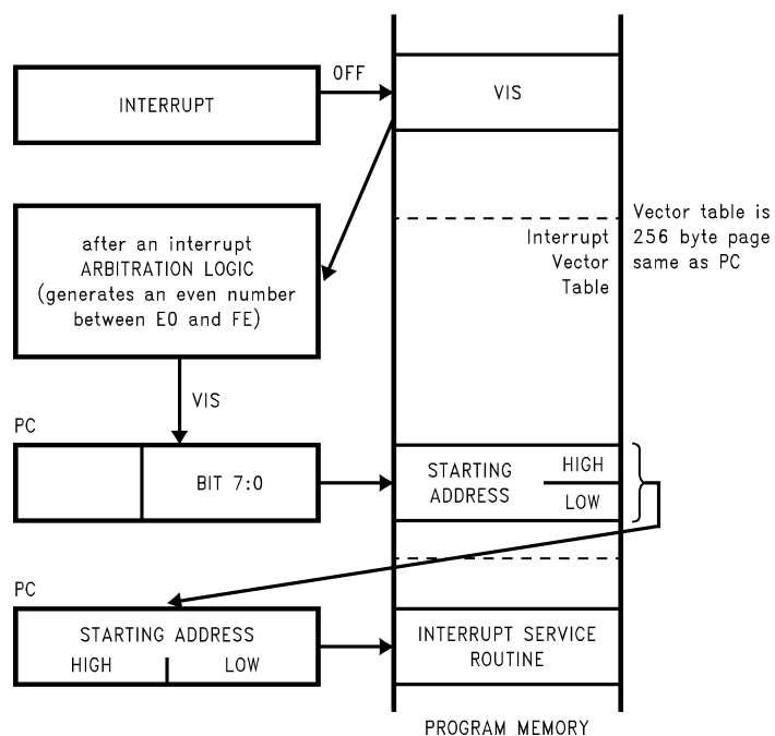
FIGURE 27. VIS Operation
