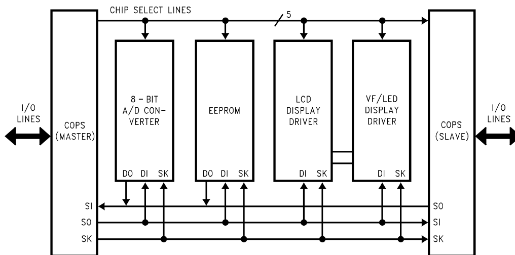
FIGURE 29. MICROWIRE/PLUS Application
