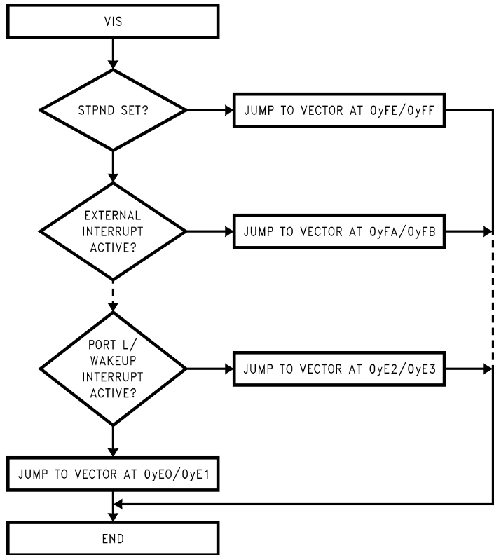
FIGURE 28. VIS Flowchart
