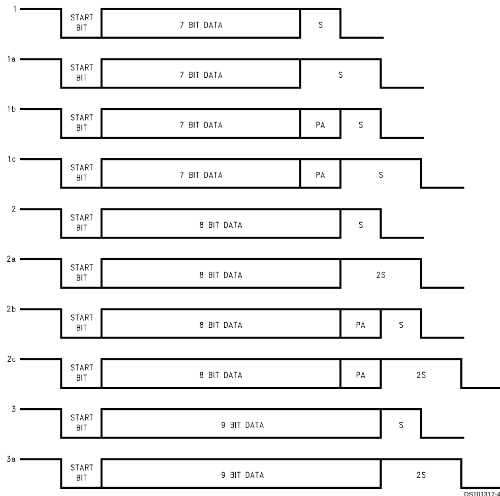
FIGURE 23. Framing Formats
