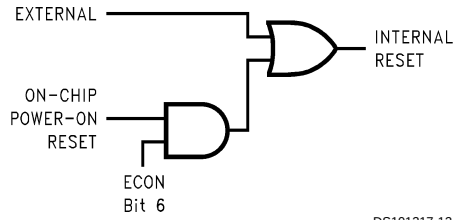
FIGURE 9. Reset Logic
