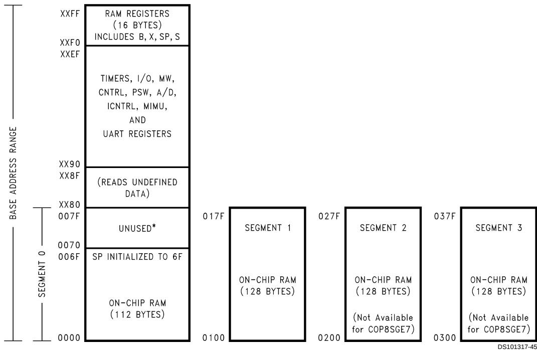
FIGURE 8. RAM Organization
