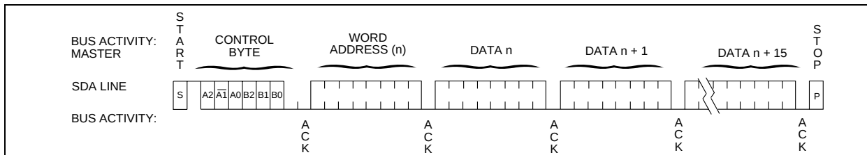
FIGURE 4-2: PAGE WRITE
