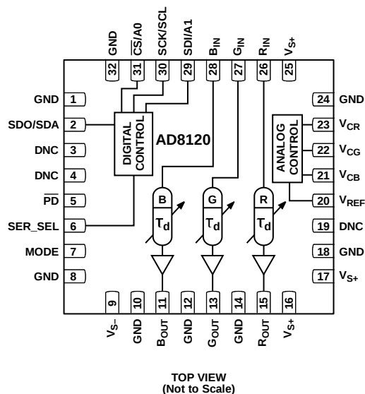
Figure 3. Pin Configuration
