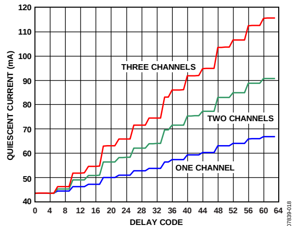
Figure 9. Quiescent Current vs. Delay Code
