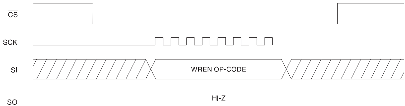
Figure 6-2. WREN Timing
