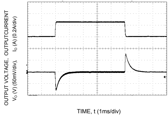
Figure 5. Transient Response to Dynamic Load Change from 50% to 75% to 50% of full load.
