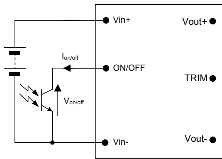
Figure 46. Circuit configuration for using Remote On/Off Implementation.
