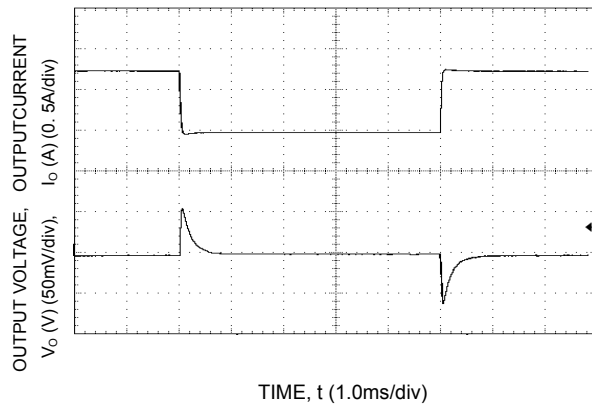
Figure 35. Transient Response to Dynamic Load Change from 50% to 75% to 50% of full load.
