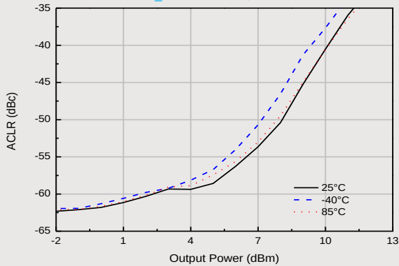
5G NR ACLR vs. Channel Power @ 3.75GHz
