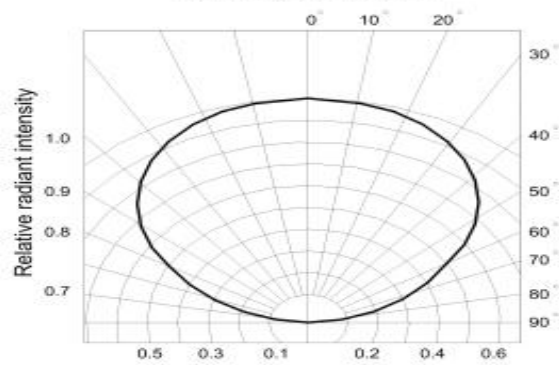
Fig.6 Radiation diagram
