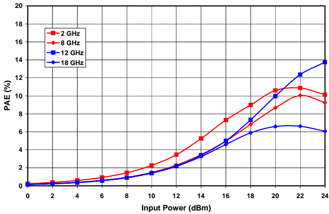
Figure 9. Power Added Efficiency vs. Input Power and Frequency at 10V and I_{DC} = 750\text{mA} .
