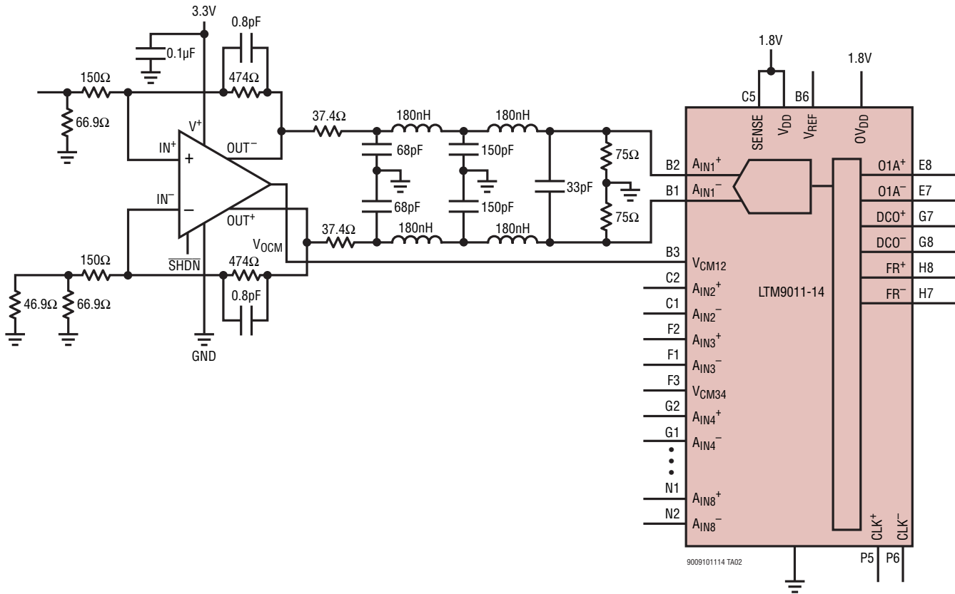
Single-Ended to Differential Conversion Using LTC6409 and 50MHz Lowpass Filter (Only One Channel Shown)
