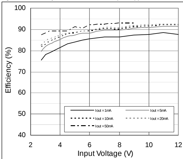
Figure 7. Efficiency vs. V_{IN} ; V_{OUT}=18V , Split Supplies
