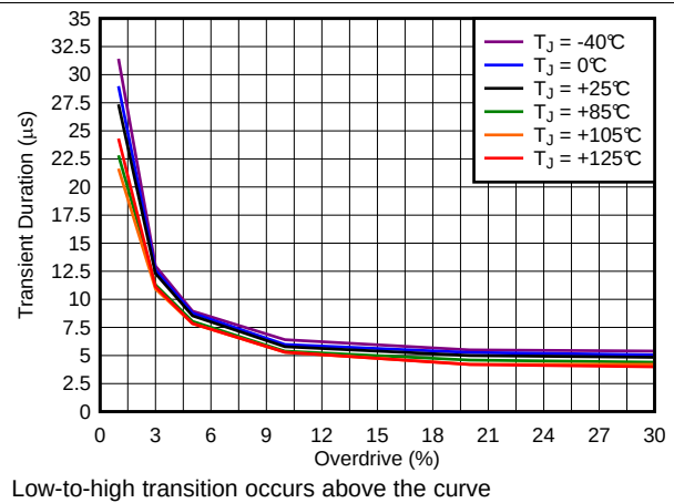
Figure 19. Minimum Transient Duration vs Overdrive (VDD = 5.5 V)
