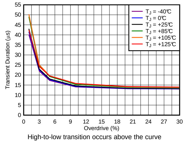
Figure 17. Minimum Transient Duration vs Overdrive (VDD = 5.5 V)
