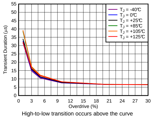
Figure 16. Minimum Transient Duration vs Overdrive (VDD = 1.5 V)
