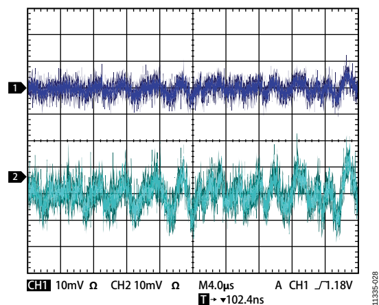
图15. 输出噪声; 测试电路1, 通道1 = EA OUT (10 mV/div), 通道2 = EA OUT2 (10 mV/div)
