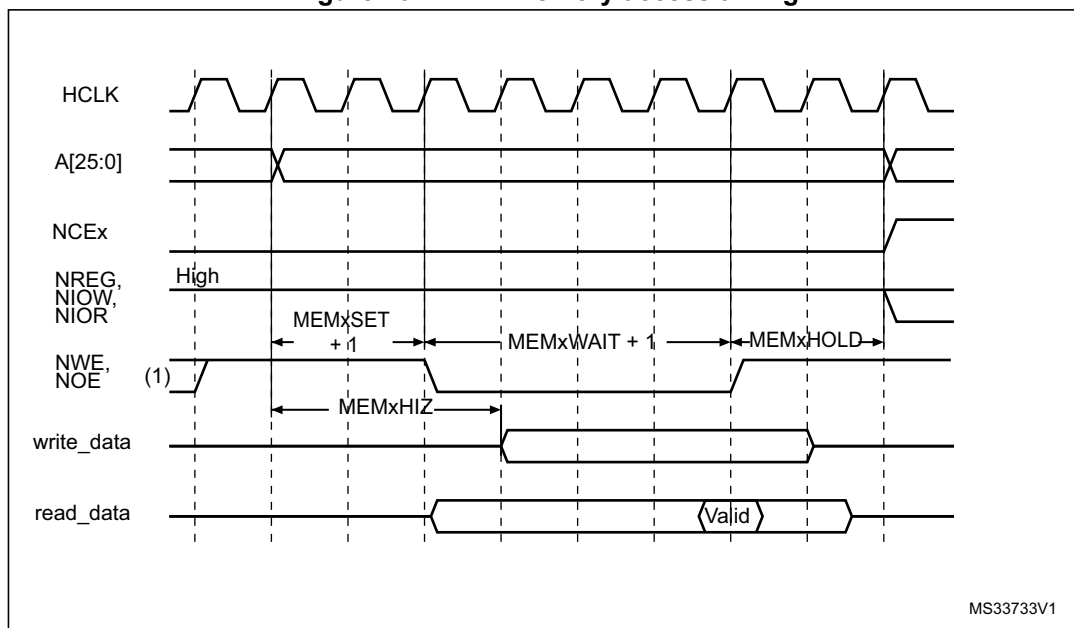
Figure 10. NAND memory access timing
