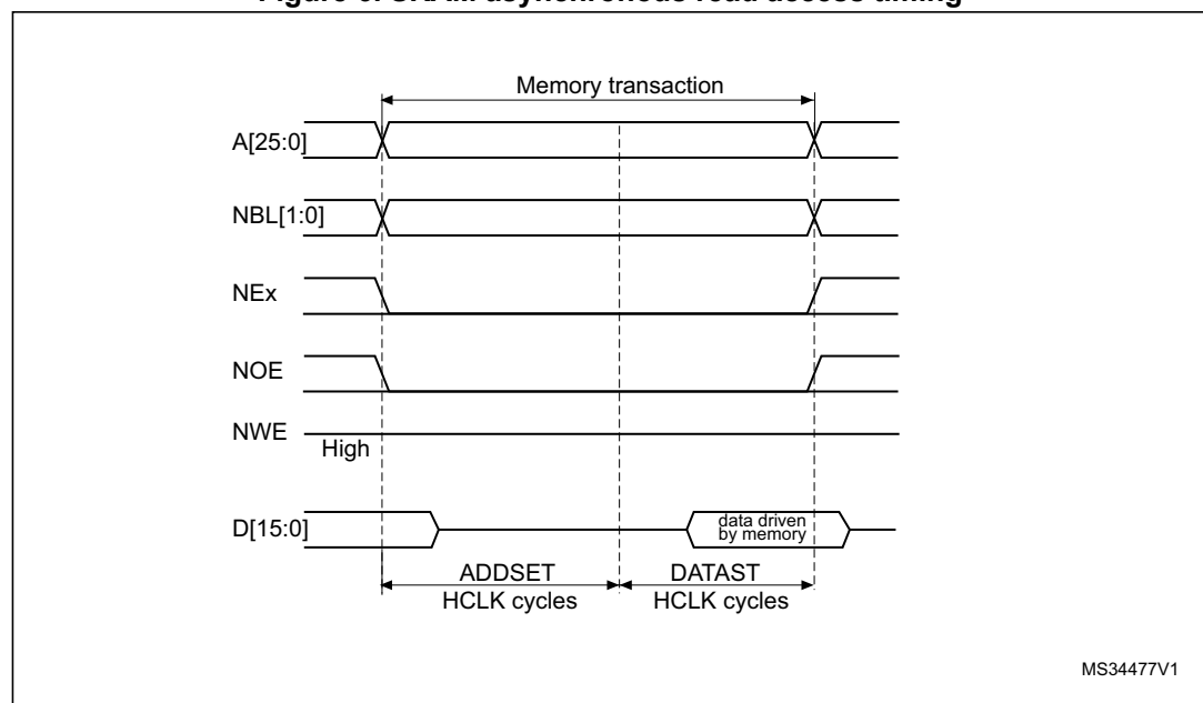
Figure 6. SRAM asynchronous read access timing
