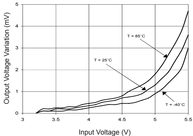
Line Regulation (Analog LD0s) Load Current = 1mA
