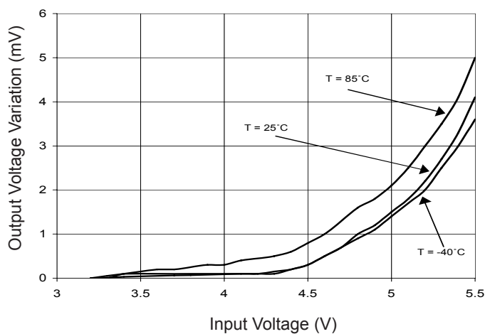
Line Regulation (Digital LD0s) Load Current = 1mA
