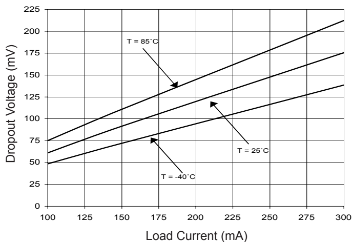
Dropout Voltage vs. Load Current (Digital LD0s)
