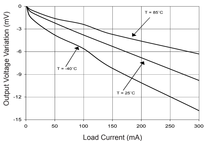
Load Regulation (Digital LD0s) VIN = 3.7V
