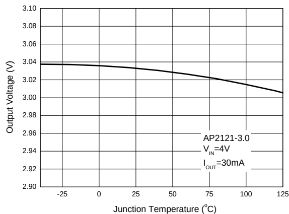
Figure 11. Output Voltage vs. Junction Temperature
