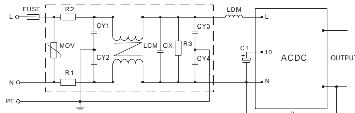
Fig. 3: PPM-SIP-Series Recommended circuit for application require higher EMC standard (external circuit output same as above)
