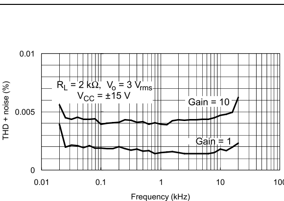
Figure 7. THD + noise vs. frequency
