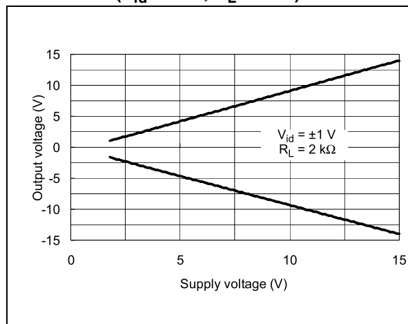
Figure 6. Output voltage vs. supply voltage ( V_{id} = \pm 1 V, R_L = 2 kΩ)
