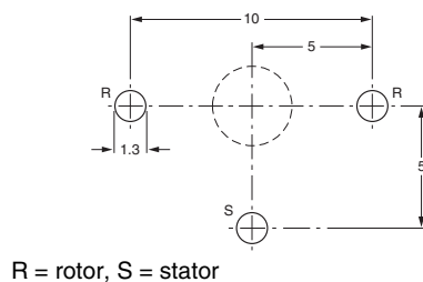
Hole pattern
