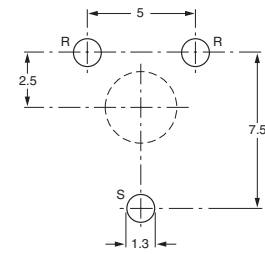
Hole pattern
