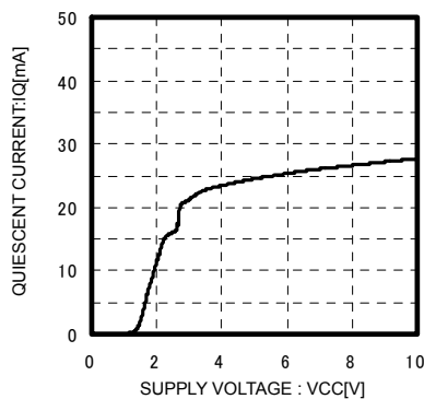
Fig.1 Iq vs Vcc
