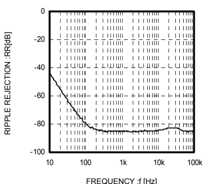
Fig.8 Ripple Rejection Ratio
