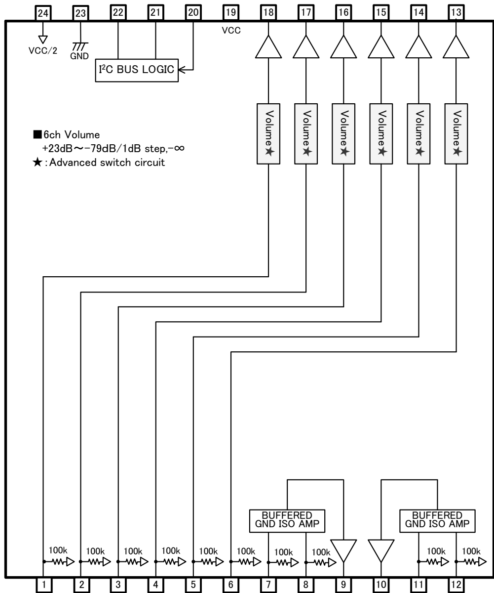
Fig.17 BD3460FS
