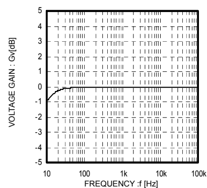
Fig.3 Gain vs Freq
