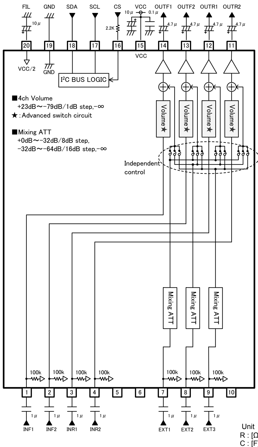
Fig.26 BD3465FV
