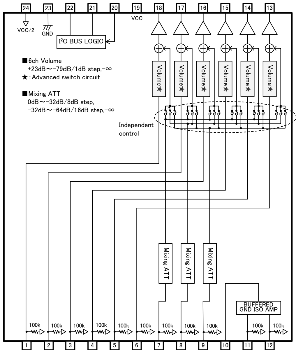
Fig.18 BD3461FS
