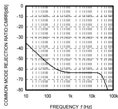
Fig.12 CMRR vs freq (BD3460FS, BD3461FS)
