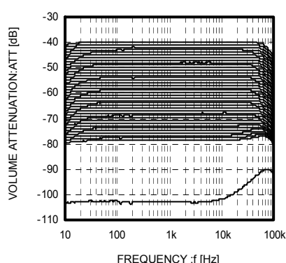
Fig.6 Volume Gain vs freq 2 (-41~-79dB)
