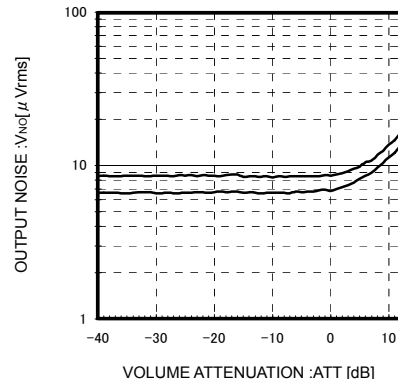
Fig.9 Volume Gain vs Noise
