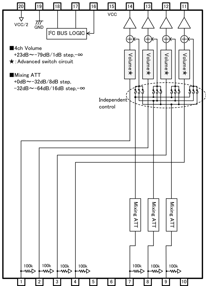
Fig.20 BD3465FV
