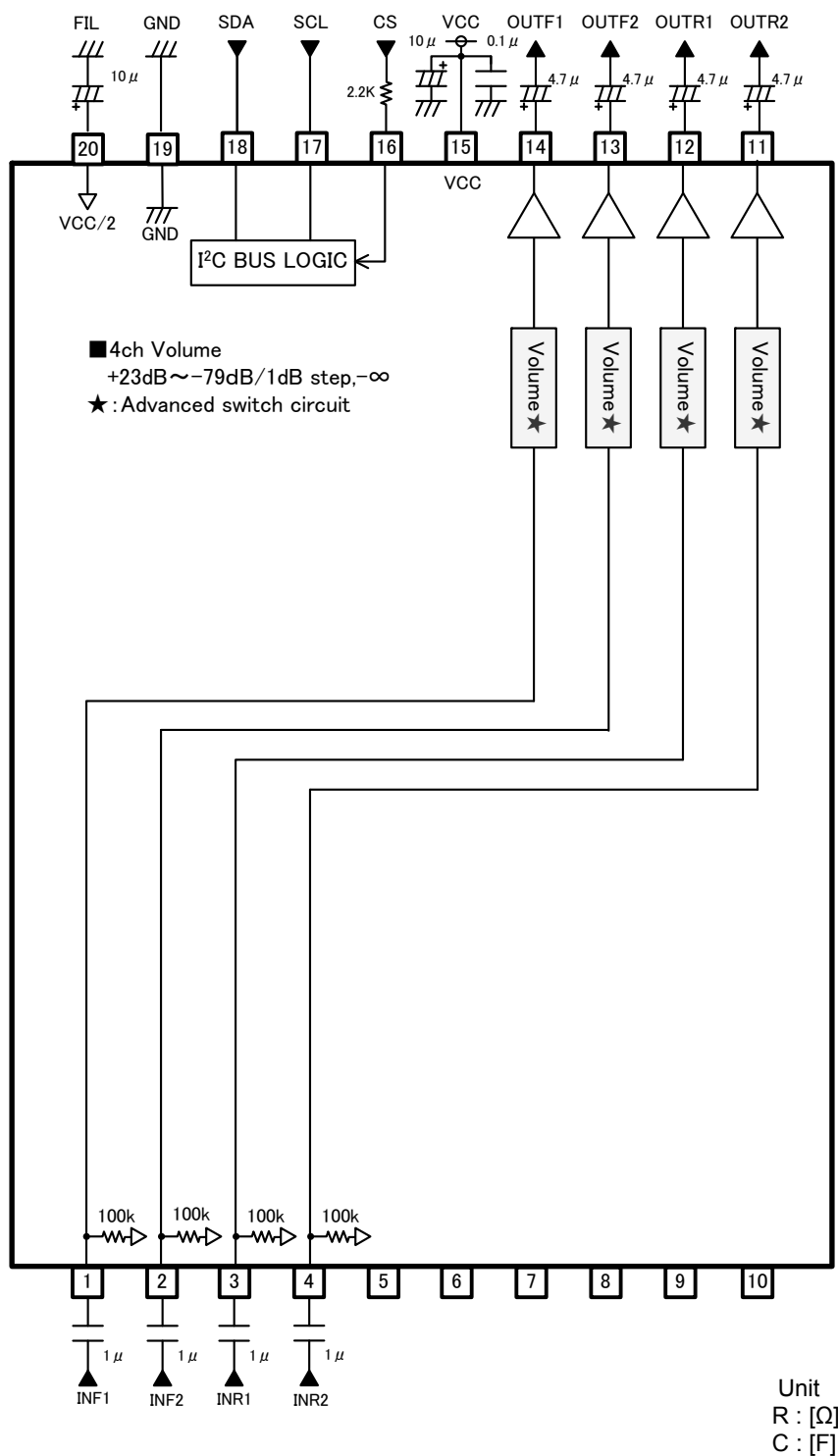
Fig.25 BD3464FV
