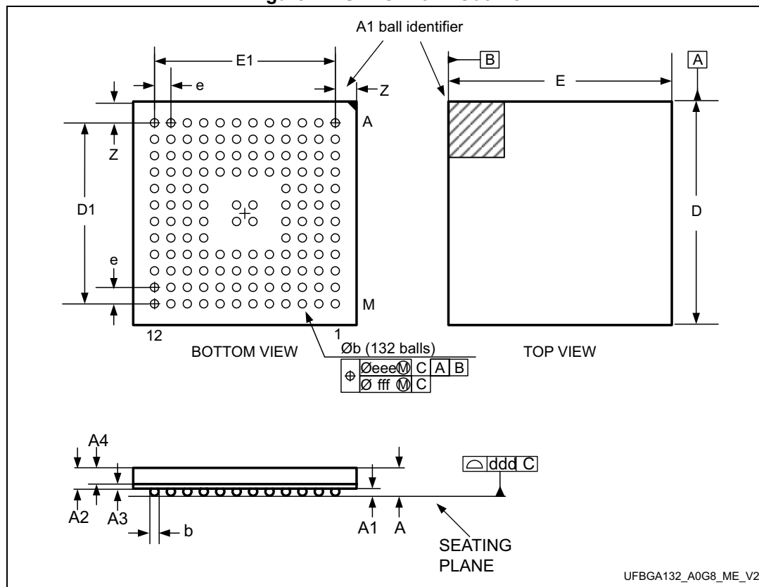
Figure 72. UFBGA132 - Outline
