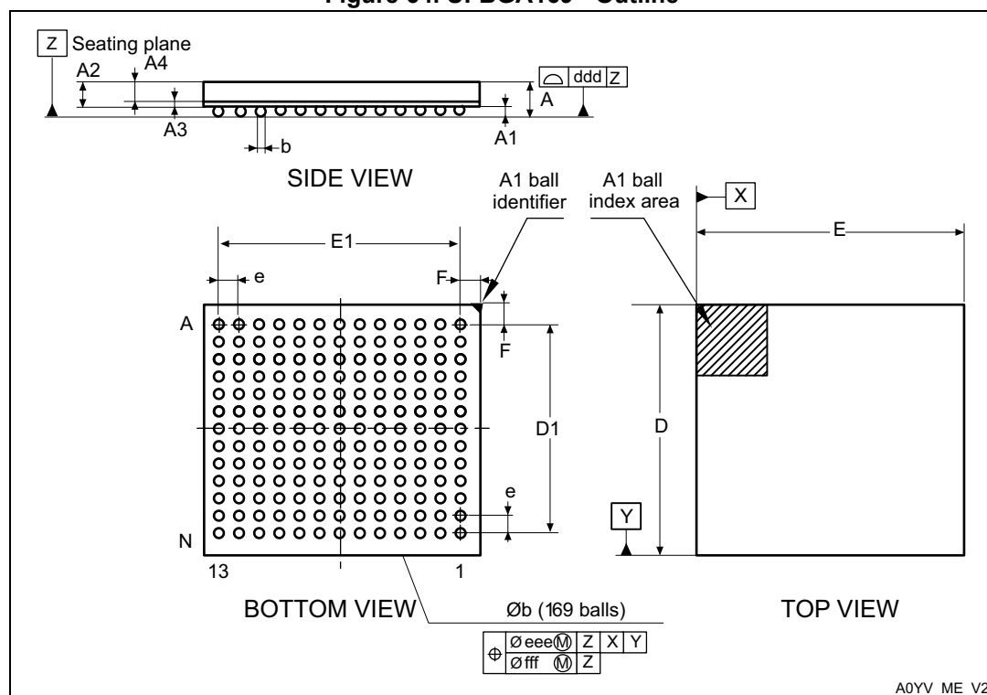
Figure 64. UFBGA169 - Outline
