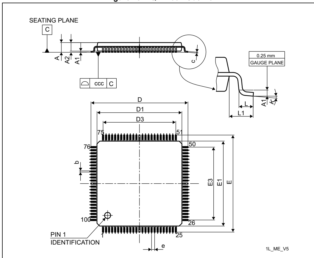
Figure 79. LQFP100 - Outline
