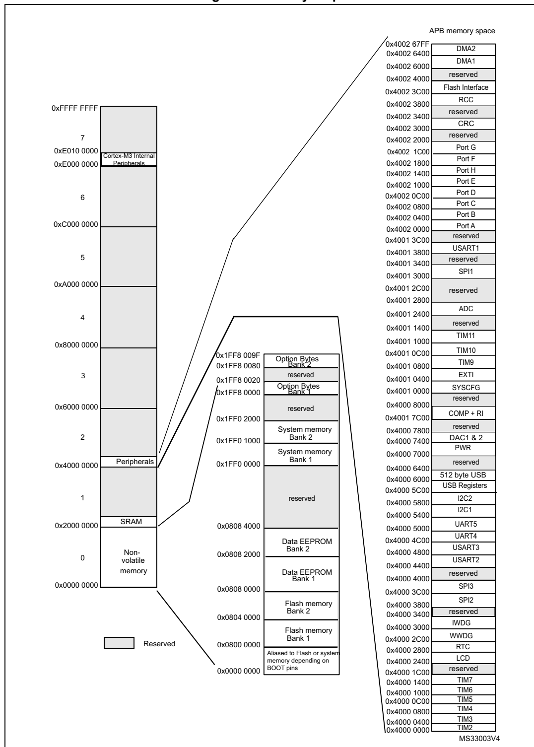
Figure 8. Memory map
