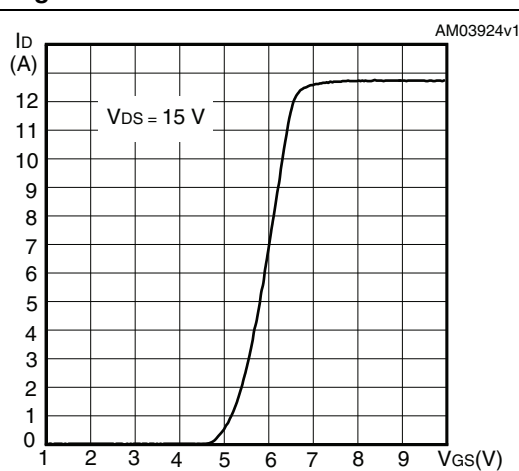
Figure 7. Transfer characteristics
