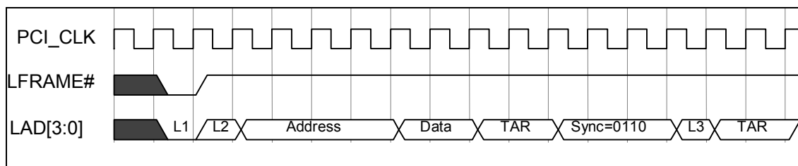
FIGURE 22 – I/O WRITE
