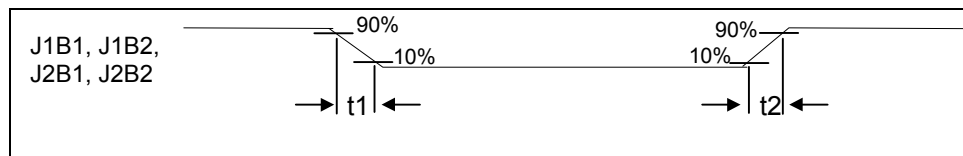
FIGURE 42 – JOYSTICK BUTTON SIGNAL
