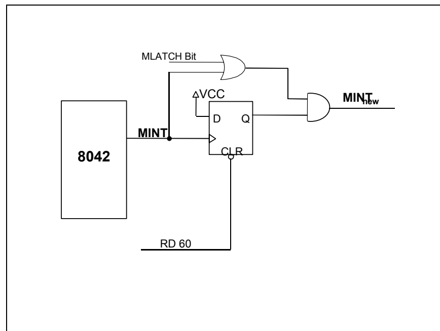
FIGURE 7 – MOUSE LATCH
