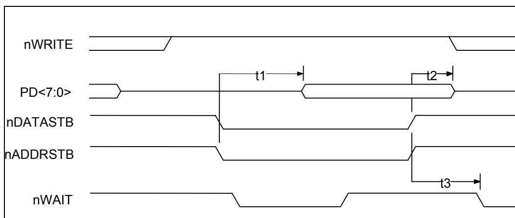
FIGURE 31 – EPP 1.7 DATA OR ADDRESS READ CYCLE
