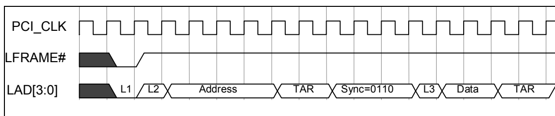
FIGURE 23 – I/O READ
