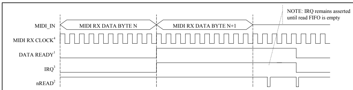
FIGURE 4 – MPU-401 INTERRUPT
