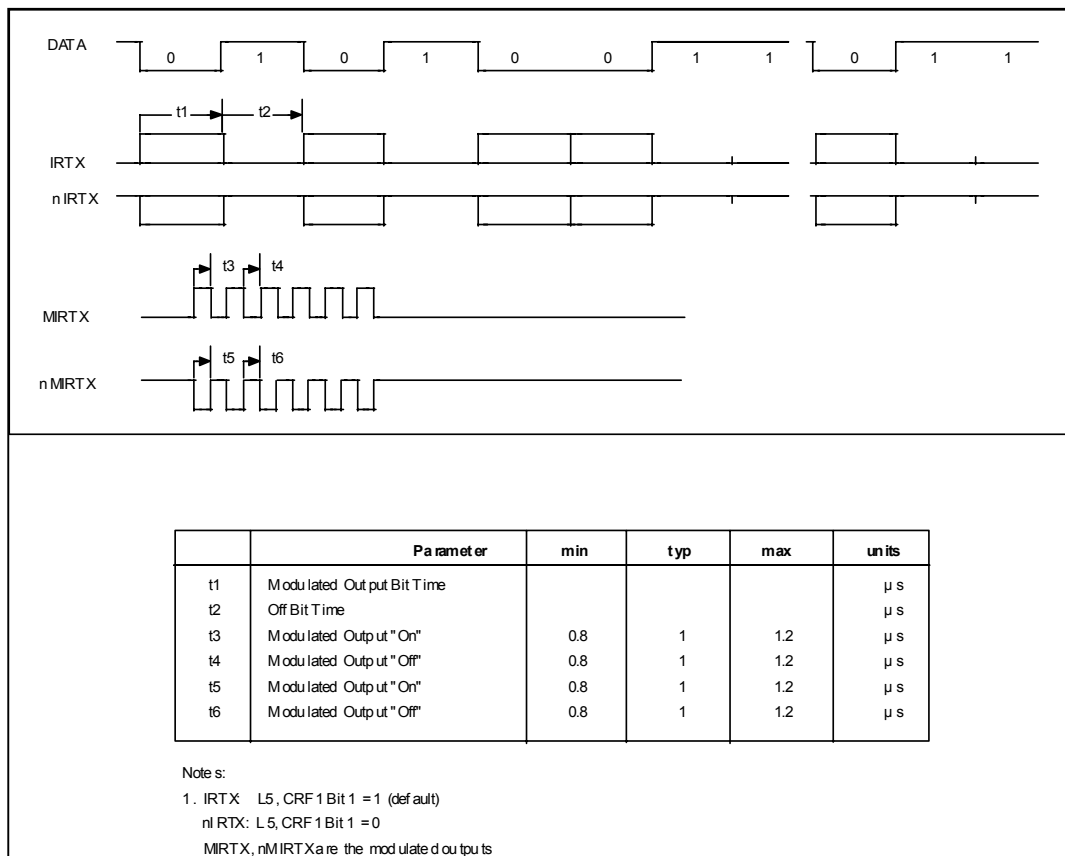
FIGURE 38 – AMPLITUDE SHIFT KEYED IR TRANSMIT TIMING
