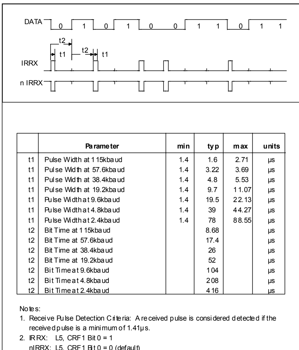
FIGURE 35 – IRDA RECEIVE TIMING
