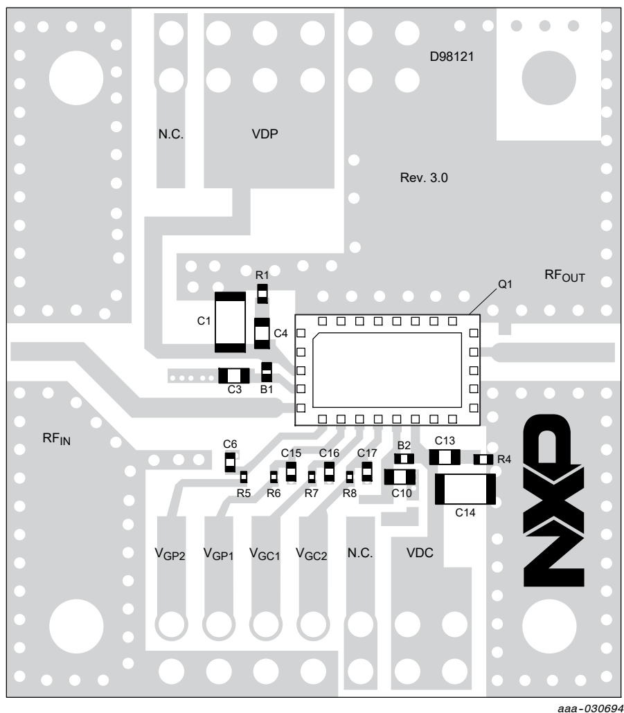
Figure 2. AFSC5G26E38 Reference Circuit Component Layout
