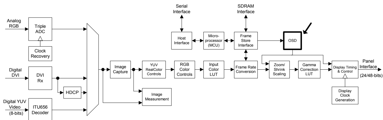
Figure 45. OSD Block
