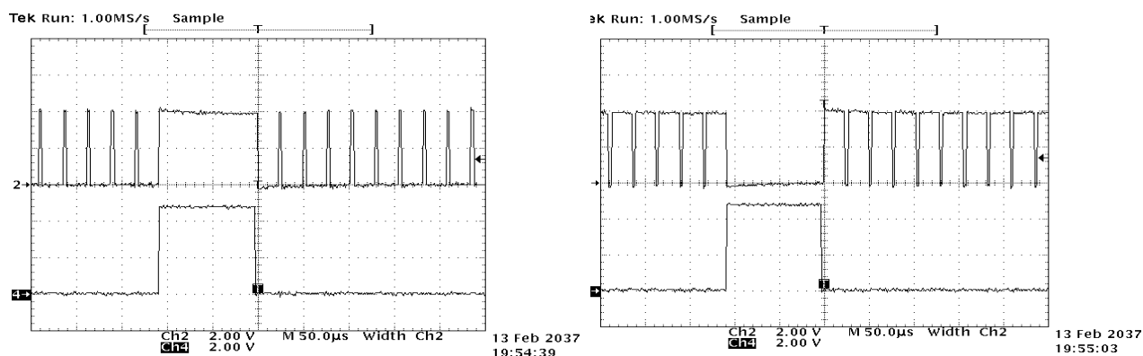
Figure 12. Positive and negative polarity OR-type CSYNC
