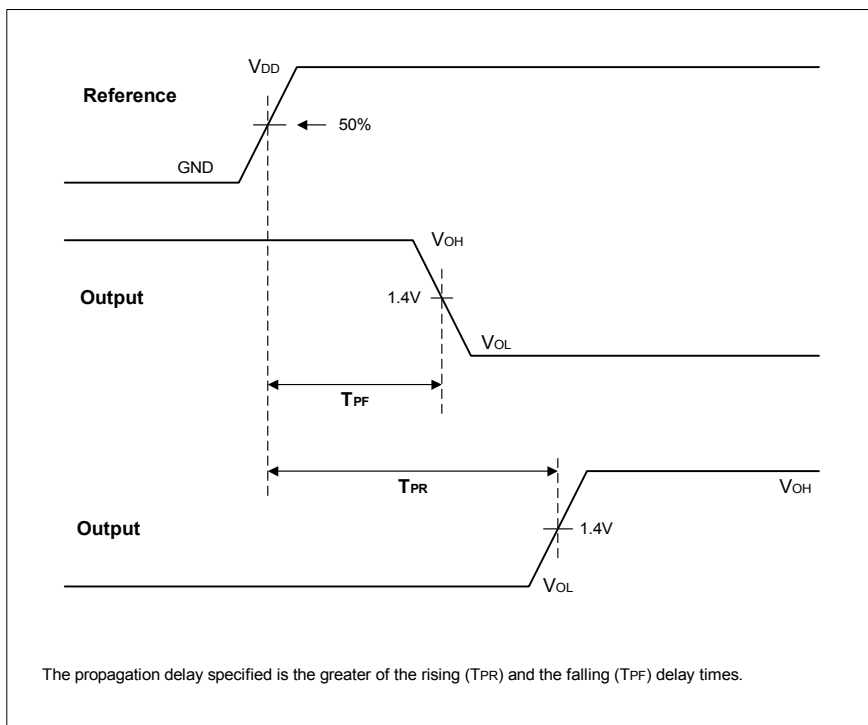
Figure 62. Propagation Delay Reference Levels
