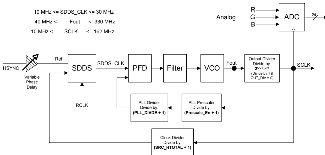
Figure 16. gm5060 Clock Recovery
