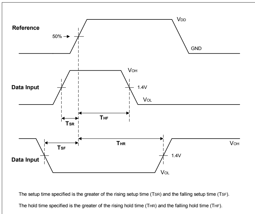
Figure 61. Setup and Hold Reference Levels
