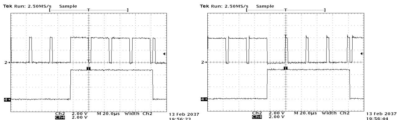
Figure 14. Positive and negative polarity serration-type CSYNC
