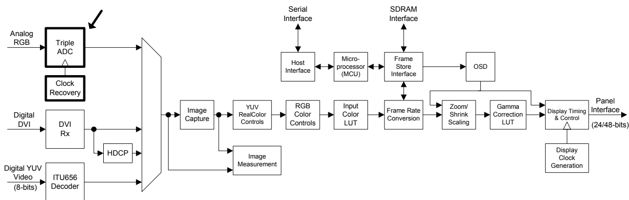
Figure 10. ADC Block
