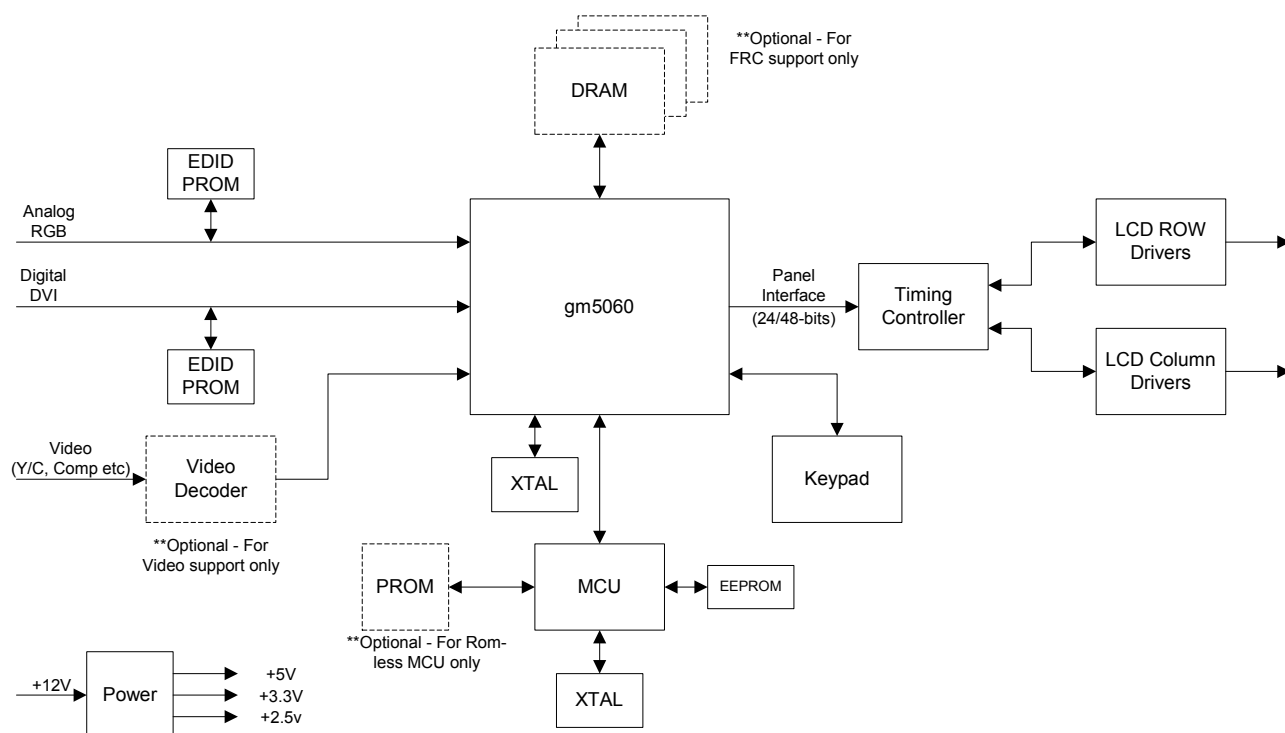
Figure 1. gm5060 System Design Example
