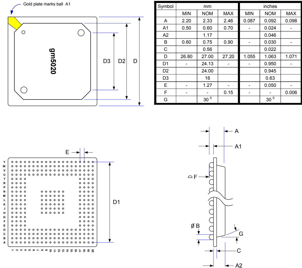
Figure 63. gm5060 292-pin PBGA
