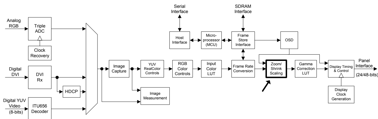
Figure 34. Scaling Block
