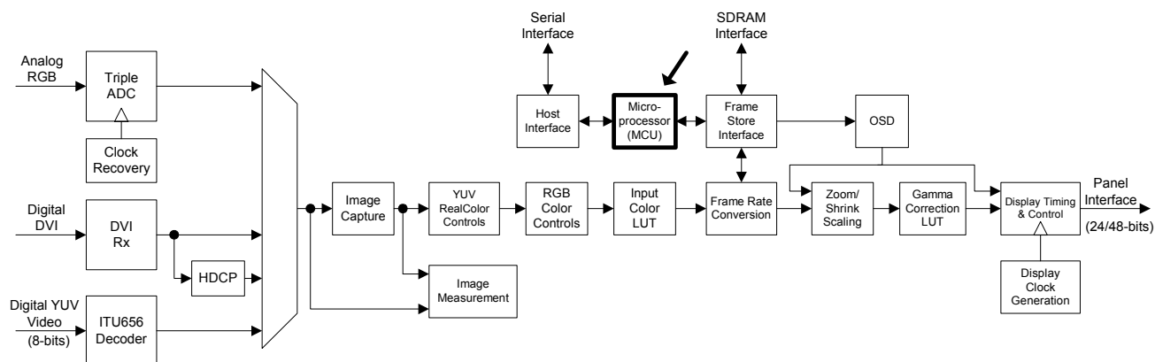
Figure 50. MCU Block
