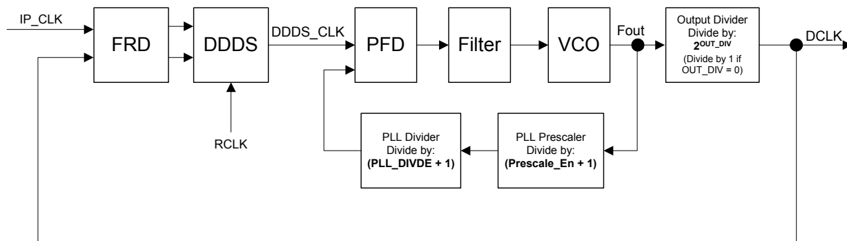
Figure 38. DDDS Block
