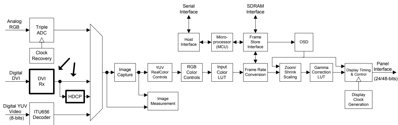
Figure 18. DVI Block
