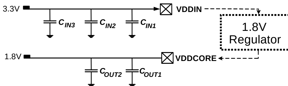
Figure 6-1. Supply Decoupling
