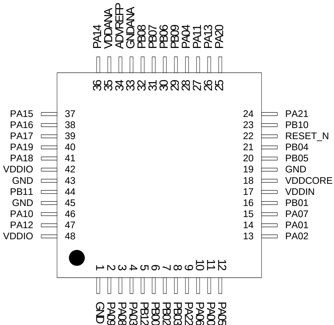
Figure 3-1. TQFP48/QFN48 Pinout
