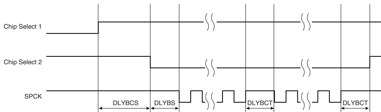
Figure 20-7. Programmable Delays
