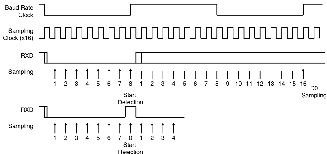
Figure 19-7. Asynchronous Character Reception
