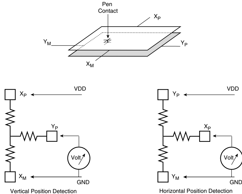
Figure 26-2. Resistive Touch Screen Position Measurement
