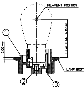
ASS'Y CONDITION
