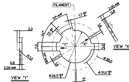
MOUNTING INTERFACE (MI-11)
