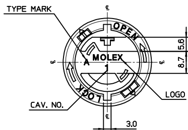
VIEW "A"
