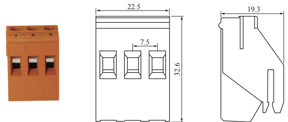
JBK5 special Crimp terminal for transformer,Spacing 7.5,Current 30A
