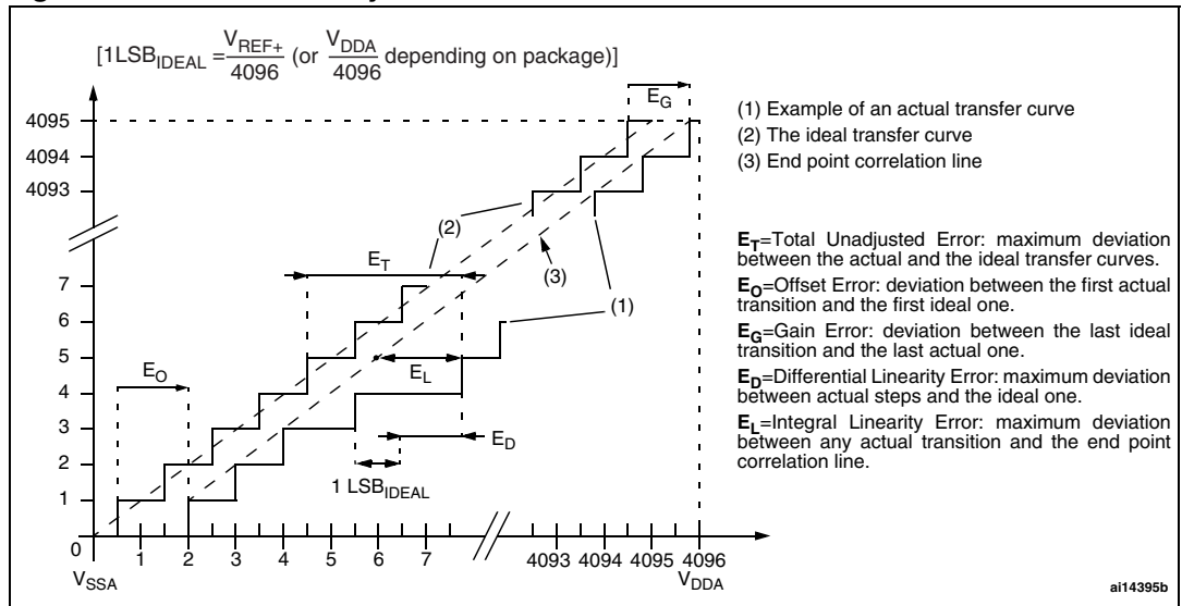
Figure 33. ADC1 accuracy characteristics
