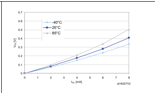
Figure 21. Typ. V_{OL} @ V_{DD} = 1.8 V (high sink ports)
