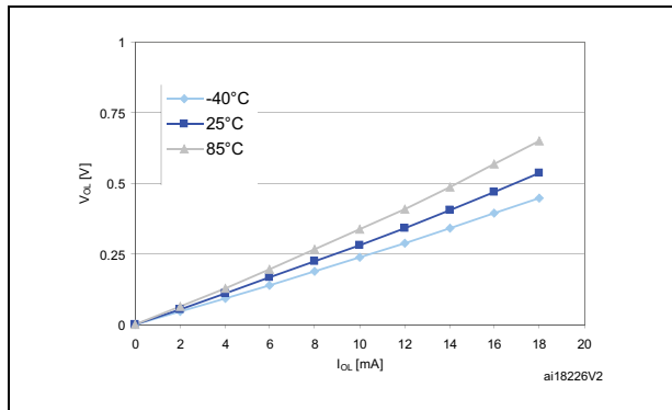
Figure 20. Typ. V_{OL} @ V_{DD} = 3.0 V (high sink ports)
