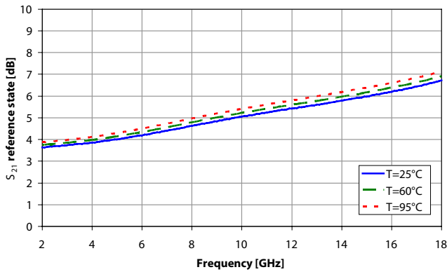
Insertion Loss vs Temp - Reference State
