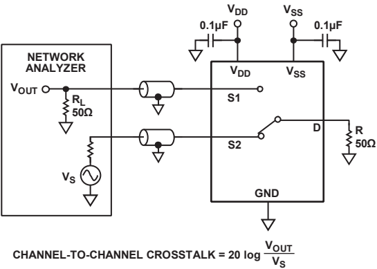
Figure 24. Channel-to-Channel Crosstalk
