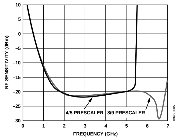
Figure 7. RF Input ( RF_{IN} ) Sensitivity
