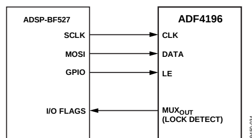
Figure 39. ADSP-BF527-to-ADF4196 Interface
