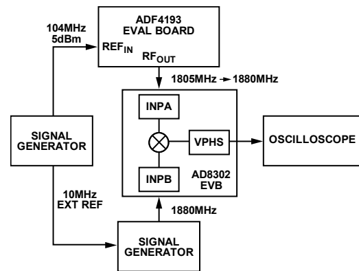
Figure 19. Test Setup for Phase Lock Time Measurements
