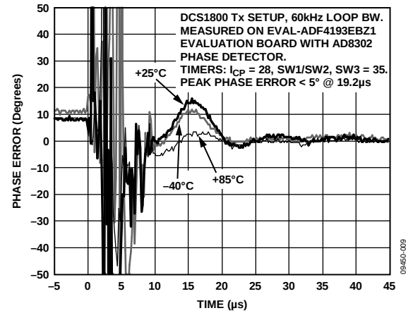
Figure 14. Phase Settling Transient for a 75 MHz Jump Down from 1893 MHz to 1818 MHz ( V_{TUNE} = 3.7 \text{ V} to 1.8 \text{ V} with Sirenza 1843T VCO)
