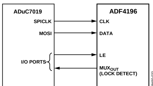
Figure 38. ADuC7019-to-ADF4196 Interface
