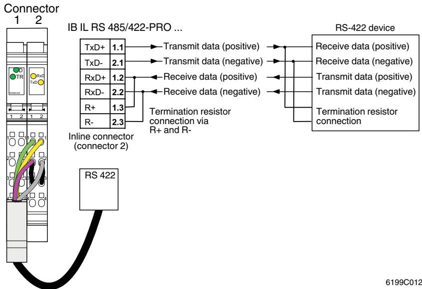
Figure 9 RS-422 interface wiring: Data line shield directly connected to FE
