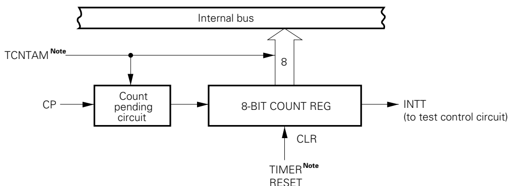
Fig. 2-12 Timer/Event Counter
