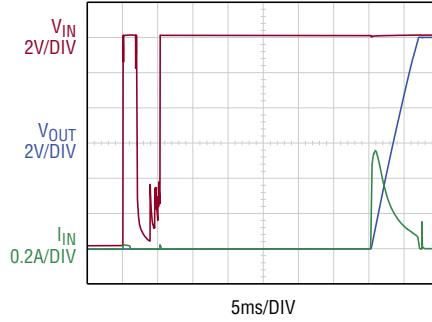
Example Hot Swap, 12V
