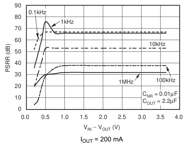
图 6-18. Power-Supply Ripple Rejection vs V_{IN} - V_{OUT}
