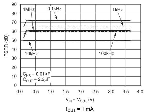
图 6-16. Power-Supply Ripple Rejection vs V_{IN} - V_{OUT}
