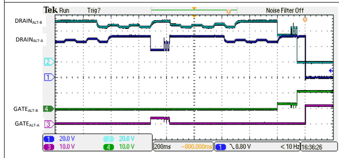
Figure 134. 4-Pair Single Signature Discovery and Turn On from Semi-Auto Mode
