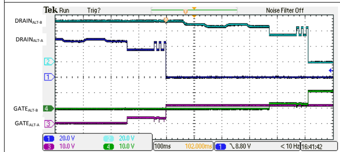
Figure 142. 4-Pair Dual Signature 3-Finger Classification and Turn On
