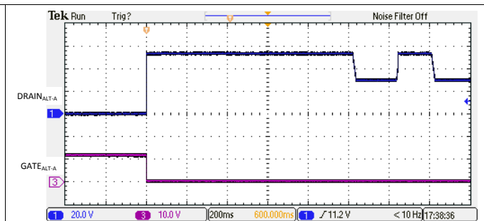
Figure 121. 2-Pair Backoff due to PCut Fault
