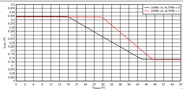
Figure 111. 1x Mode (2xFBn = 0) Foldback Curves, I PORT vs V DRAIN
