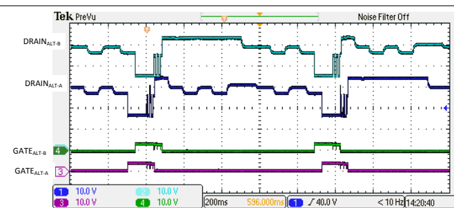
Figure 139. 4-Pair Semi-Auto Mode Discovery with a Valid Dual Signature Class 4D Load
