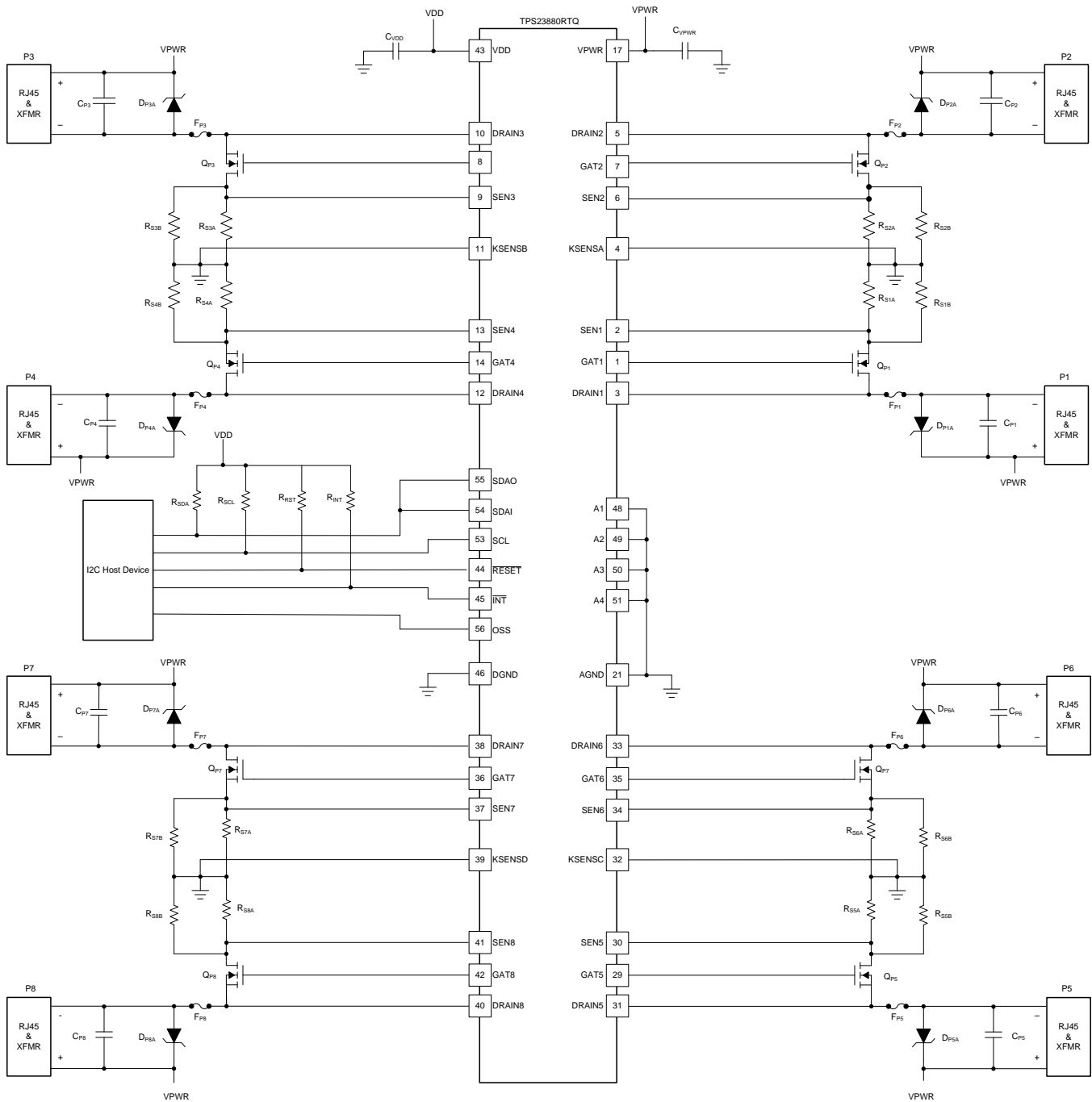
Figure 117. Eight 2-Pair Port Application
