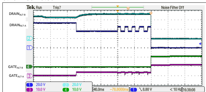
Figure 138. 4-Pair Single Signature 5-Finger Classification and Turn On
