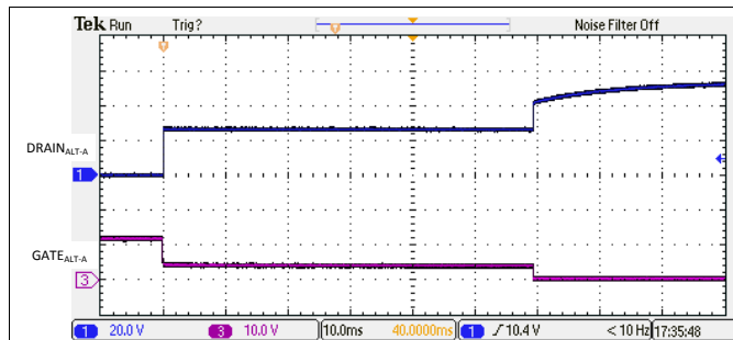
Figure 120. 2-Pair I_{LIM} Foldback and Turn Off
