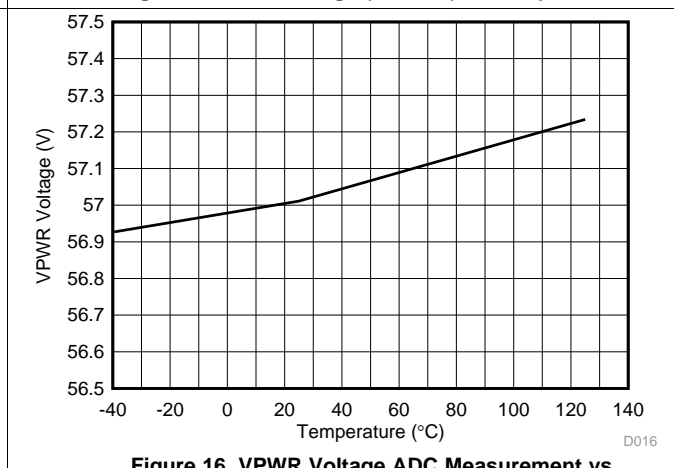
Figure 16. VPWR Voltage ADC Measurement vs Temperature
