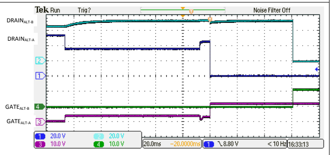
Figure 135. 4-Pair Single Signature 1-Finger Classification and Turn On
