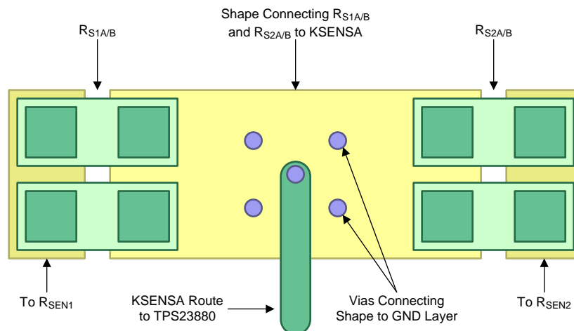
Figure 145. Kelvin Sense Layout Example
