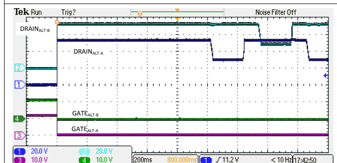
Figure 124. 4-Pair Backoff Due to 4PPCut Fault
