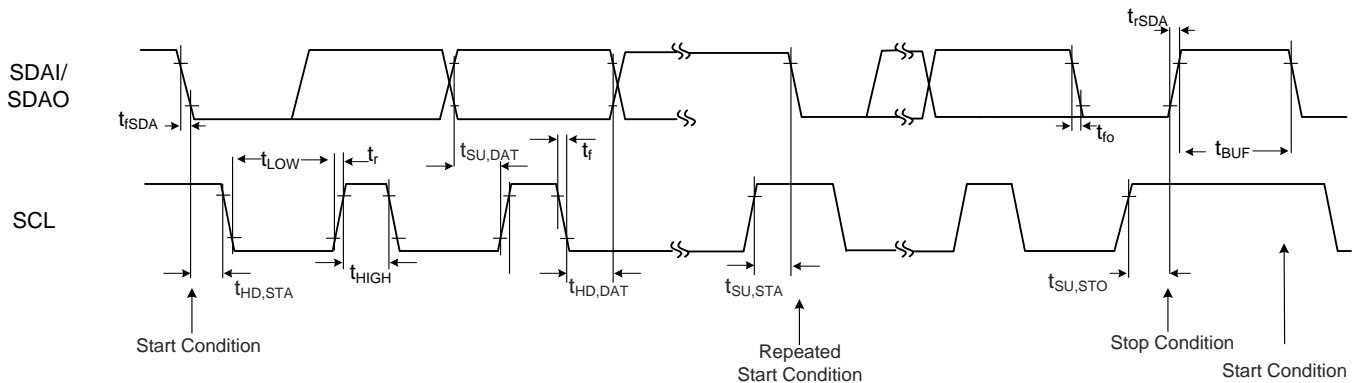
Figure 31. I 2 C Timings
