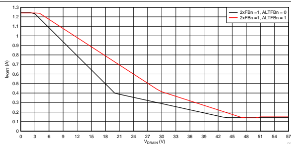
Figure 112. 2x Mode (2xFBn = 1) Foldback Curves, I PORT vs V DRAIN
