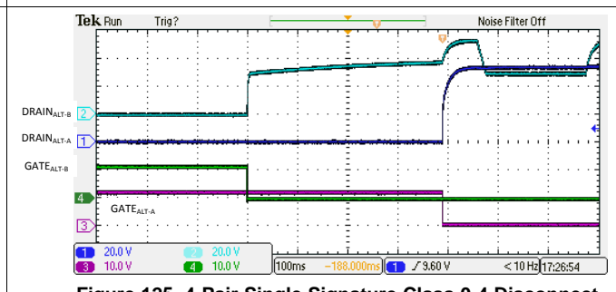
Figure 125. 4-Pair Single Signature Class 0-4 Disconnect
