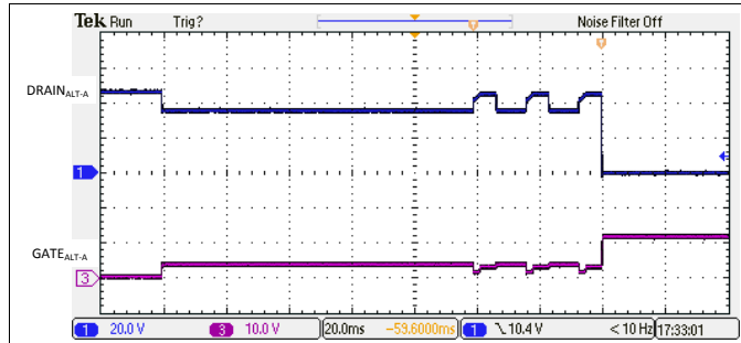
Figure 132. 2-Pair 3-Finger Classification and Turn On
