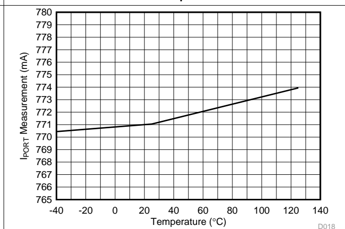
Figure 18. Port Current ADC Measurement (770mA) vs Temperature
