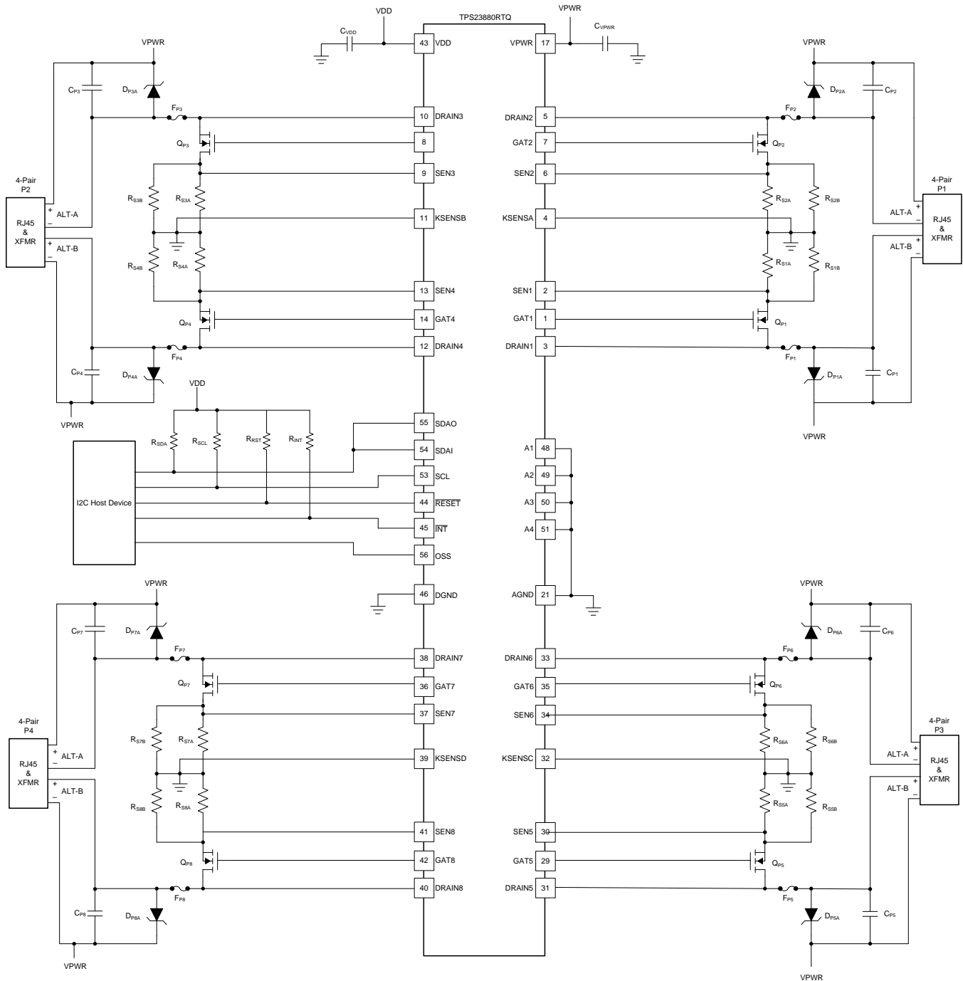
Figure 118. Four 4-Pair Port Application
