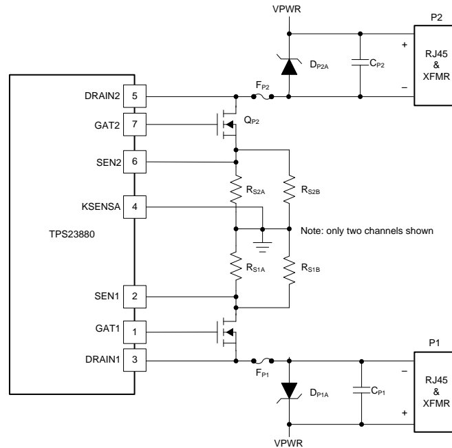
Figure 144. Kelvin Current-Sense Connection
