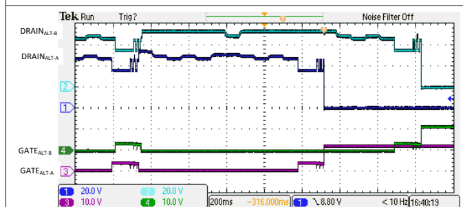
Figure 140. 4-Pair Dual Signature Discovery and Turn On from Semi-Auto Mode
