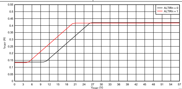
Figure 113. Inrush Foldback Curves, I PORT vs V PORT
