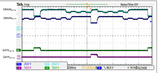
Figure 133. 4-Pair Semi-Auto Mode Discovery with a Valid Single Signature Class 0-3 Load
