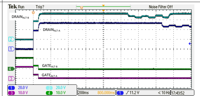
Figure 123. 4-Pair Backoff Due to I_{LIM} Fault
