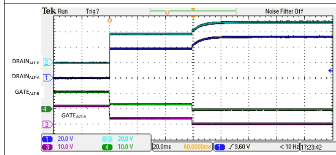
Figure 122. 4-Pair I_{LIM} Foldback and Turn Off
