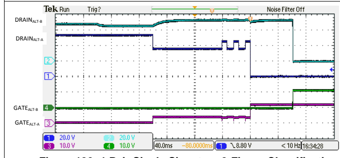
Figure 136. 4-Pair Single Signature 3-Finger Classification and Turn On
