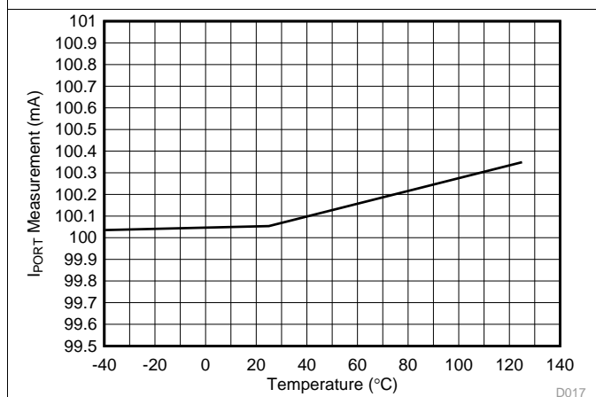
Figure 17. Port Current ADC Measurement (100mA) vs Temperature
