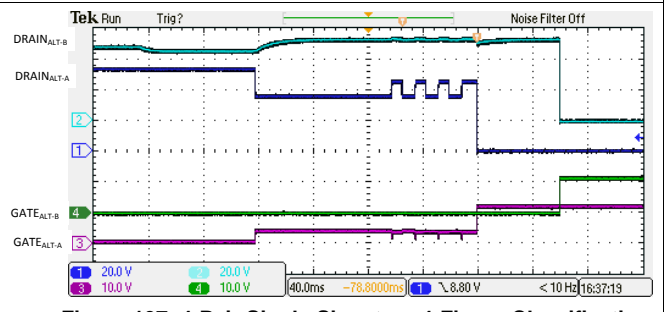
Figure 137. 4-Pair Single Signature 4-Finger Classification and Turn On
