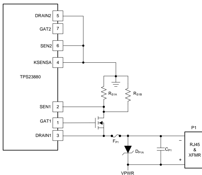
Figure 119. Unused PORT2 Connections
