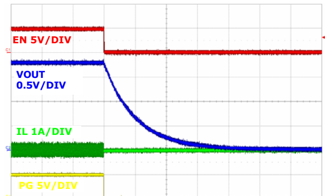
FIGURE 26. SOFT-DISCHARGE SHUTDOWN, (2ms/DIV)
