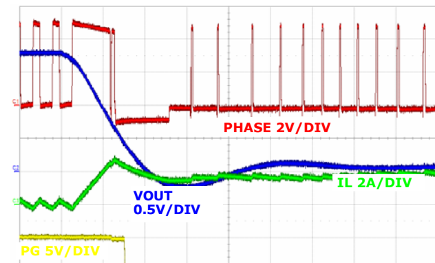
FIGURE 29. OUTPUT SHORT CIRCUIT, (500 \mu\text{s} /DIV)
