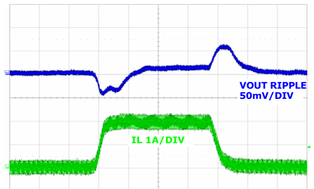
FIGURE 20. LOAD TRANSIENT (PWM), (50 \mu\text{s} /DIV)
