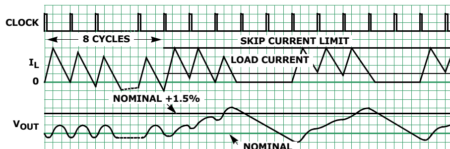
FIGURE 33. SKIP MODE OPERATION WAVEFORMS
