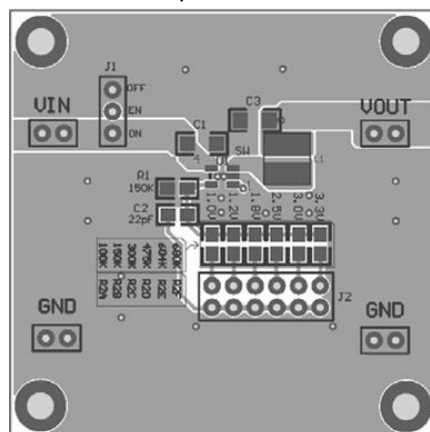
Figure 2. A7121A Suggested Layout
