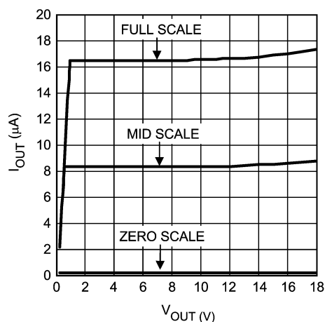
I_{OUT} vs. V_{OUT}
