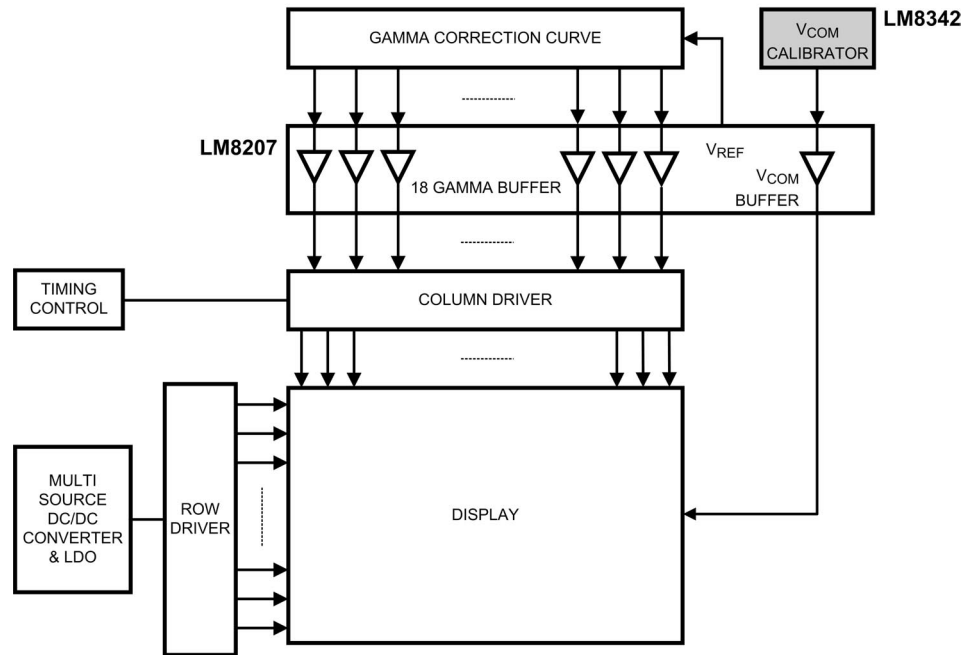
FIGURE 3. TFT Panel Block Diagram
