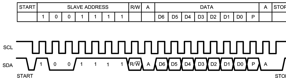
FIGURE 6. Timing Diagram
