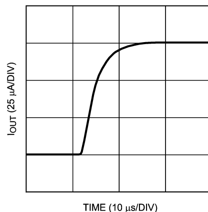
I_{OUT} Current Step Positive (Full Scale)
