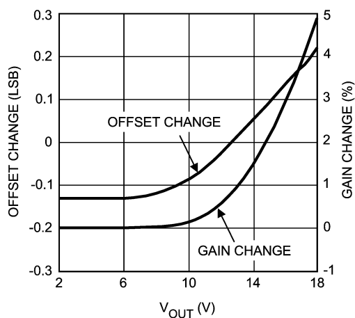
Gain & Offset Change vs. V_{OUT}
