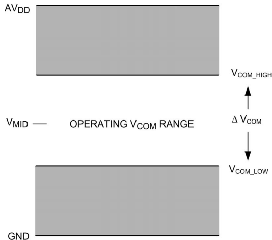
FIGURE 9. V_{COM} Voltage Levels
