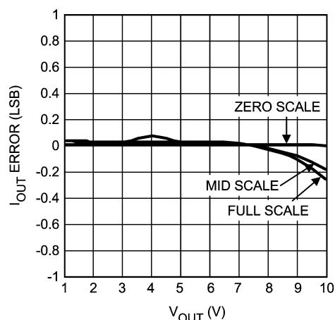
I_{OUT} Error vs. V_{OUT}
