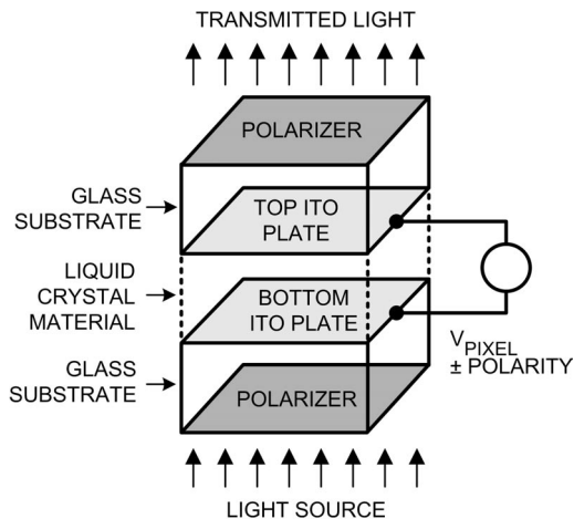
FIGURE 1. Individual LCD Pixel
