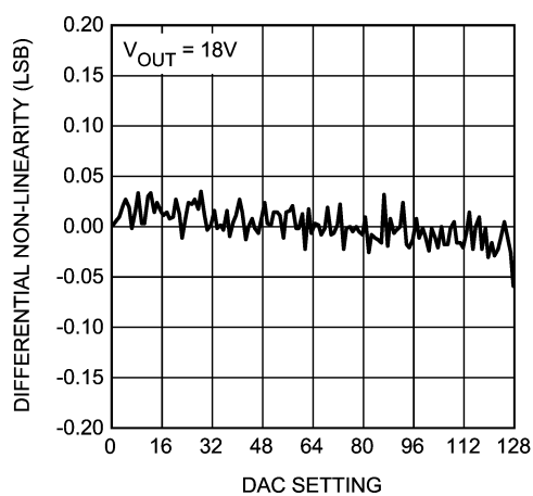
Differential Non-Linearity Error vs. DAC ( V_{OUT} = 18\text{V} )
