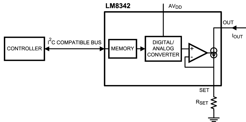
FIGURE 4. Block Diagram of the LM8342
