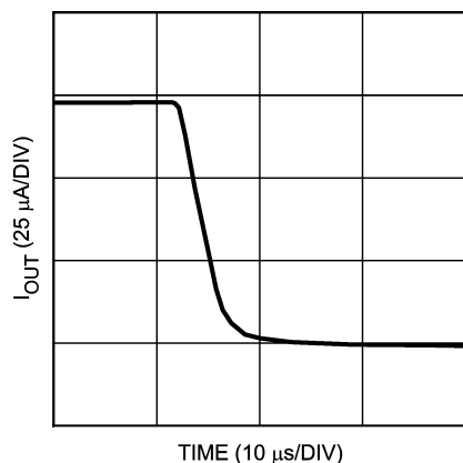
I_{OUT} Current Step Negative (Full Scale)
